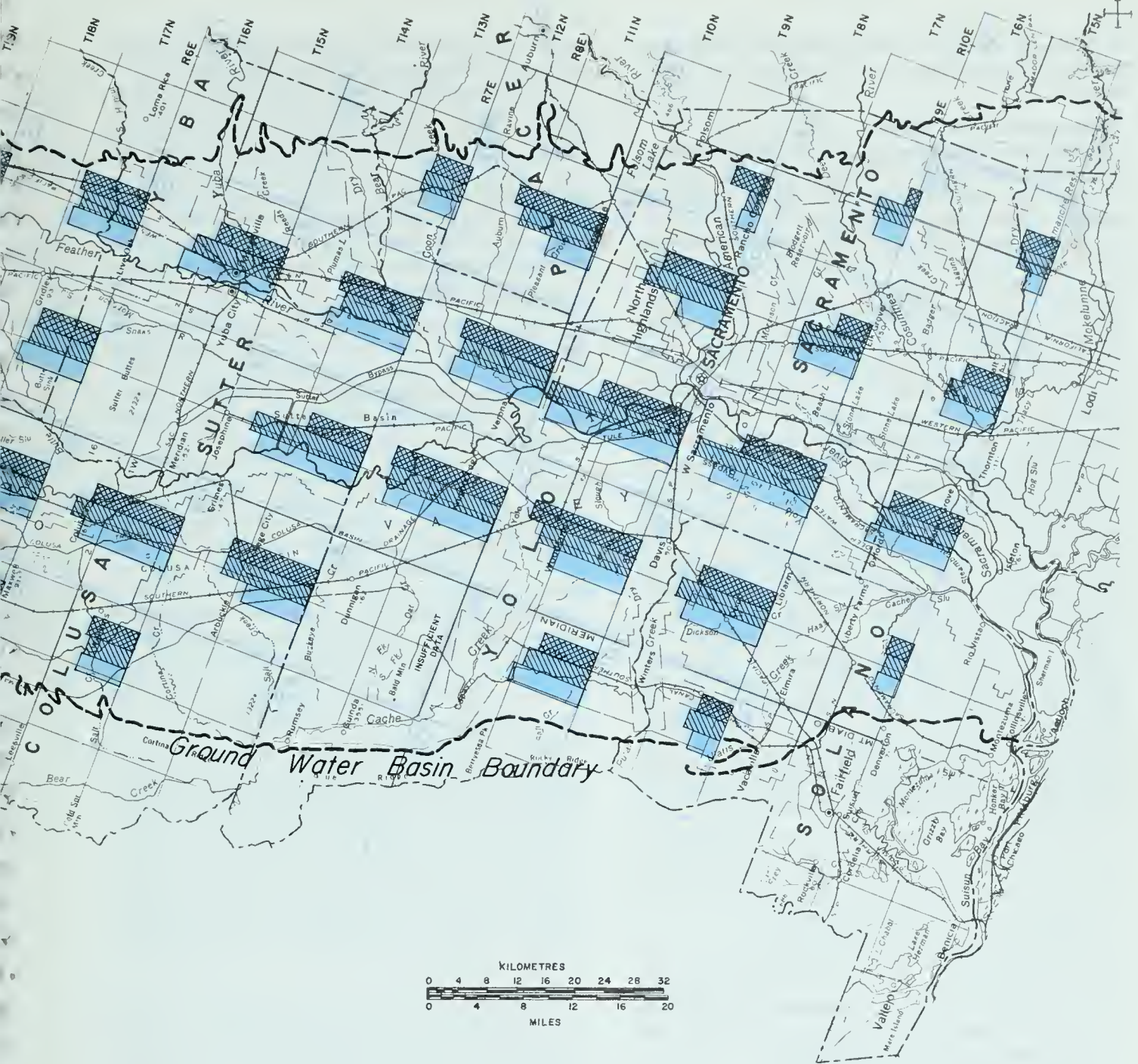
GROUND WATER IN STORAGE By Four-Township Areas 1965
