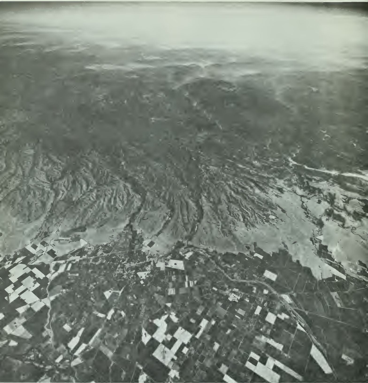
East side of Sacramento Valley at Chico. Tuscan Formation sedimentary rocks visible in foothills and Lake Almanor in the distance.
